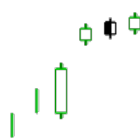
Bearish Breakaway
