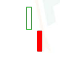
Bearish Kicking
