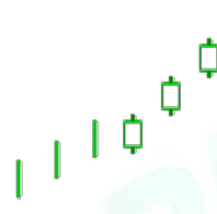
Bearish 4Gap
