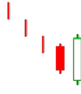
Bullish Engulfing
